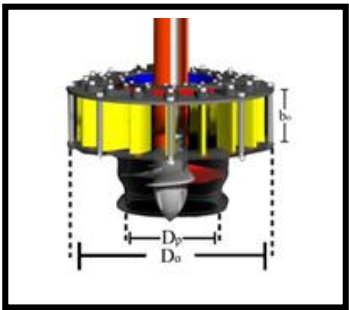
Turbin
