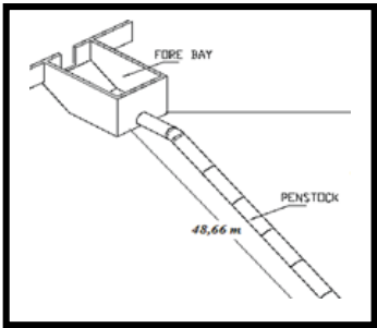
Penstock
