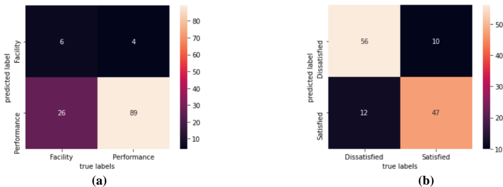
Fig. 8. Confusion matrix of Category (a) and Sentiment (b) for Scenario I
