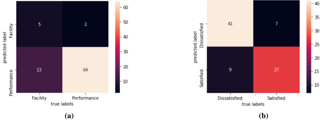
Fig. 10. Confusion matrix of Category (a) and Sentiment (b) for Scenario III
