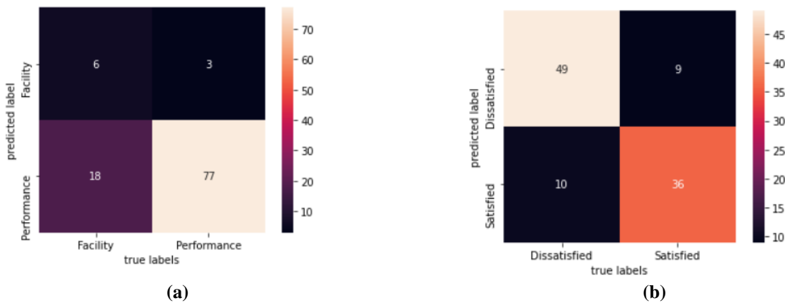
Fig. 9. Confusion matrix of Category (a) and Sentiment (b) for Scenario II
