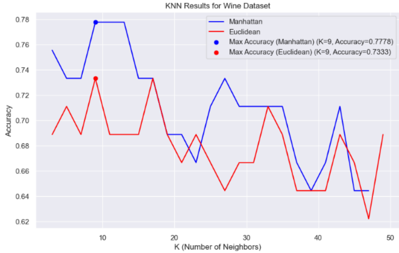
Figure 11. KNN Results for Wine Dataset
