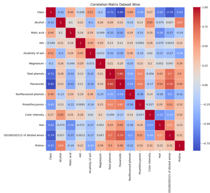
Figure 3. Correlations Matrix of dataset Wine
