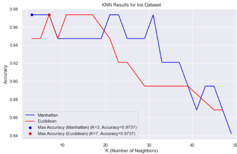
Figure 10. KNN Results for Iris Dataset
