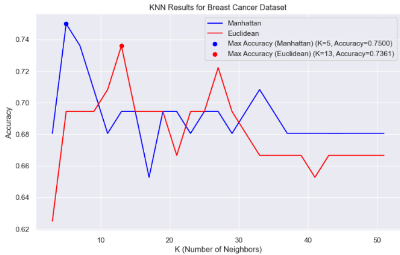
Figure 12. KNN Results for Breast Cancer Dataset
