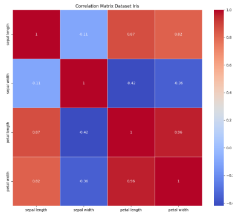
Figure 7. Correlations Matrix of dataset Iris
