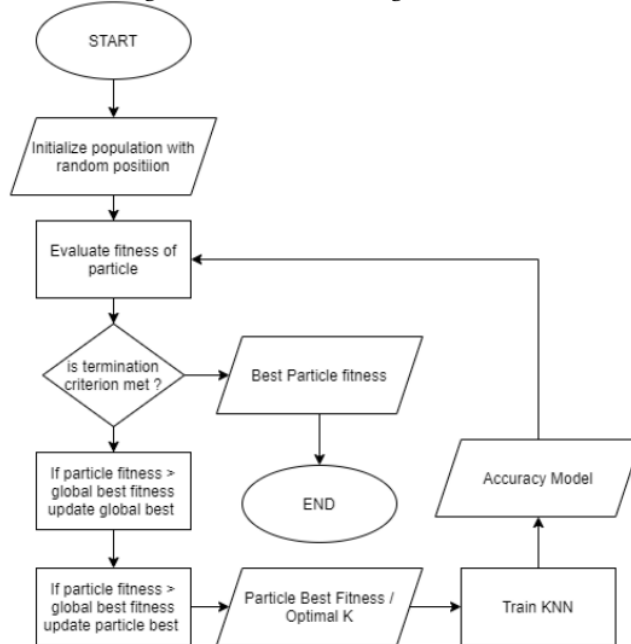
Figure 8. Flowchart PSO-KNN
