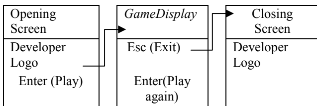
Gambar 1. Diagram alir user interface game dakon
