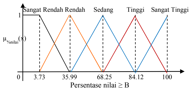
Gambar 8. Himpunan fuzzy persentase nilai mata kuliah minimal B (nilai ≥ B)
