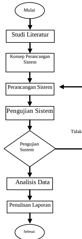
Gambar 4 Flowchat Penelitian
